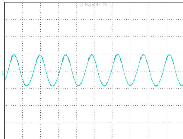
Figure 14: Output voltage ripple at nominal input voltage and rated load current ( I_o=25\text{A} ) ( 50\text{mV/div} , 2\mu\text{s/div} ) Load capacitance: 220\mu\text{F} (Electrolytic) + 10\mu\text{F} (Tantalum) + 1\mu\text{F} (Ceramic) and min Co. Bandwidth: 20\text{MHz} .
